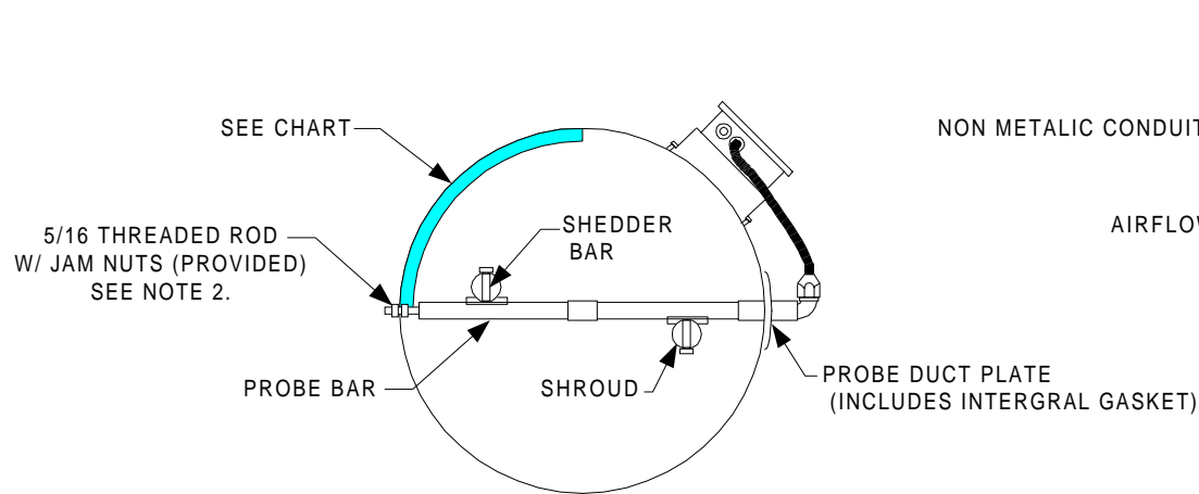
DUCT CROSS SECTION
