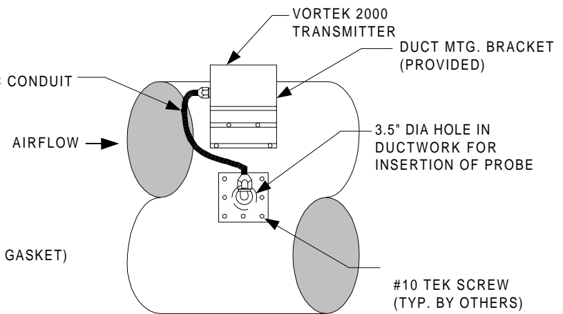
MOUNTING INSERTION PROBE
