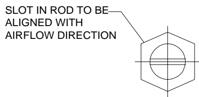
SECTION A-A PROBE ALIGNMENT SLOT REQUIRED FOR ALL BARS.
